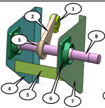
Pressing arm front/rear support plate group
