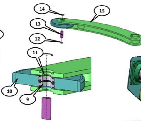
Pressing arm roller group
