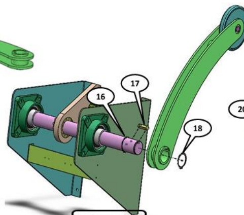
Pressing arm parts
